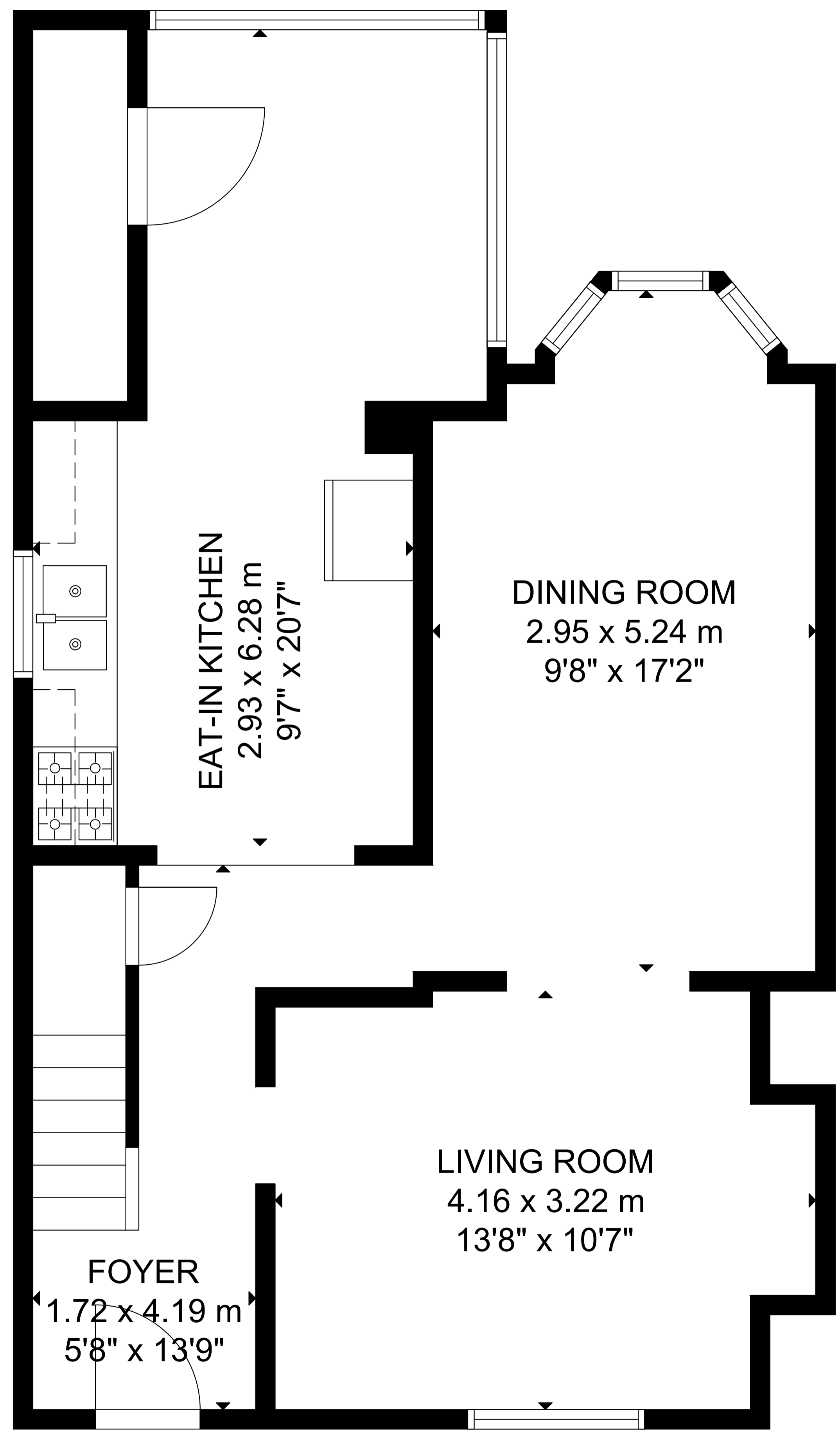
MAIN FLOOR
