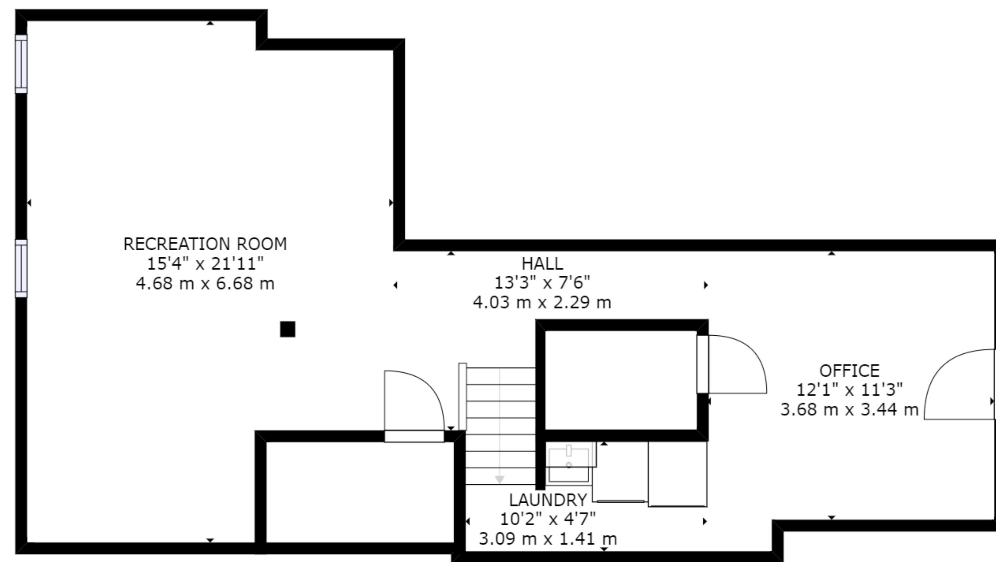
FLOOR 1
