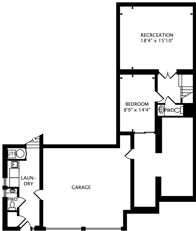
LOWER FLOOR 1179 SQUARE FEET
