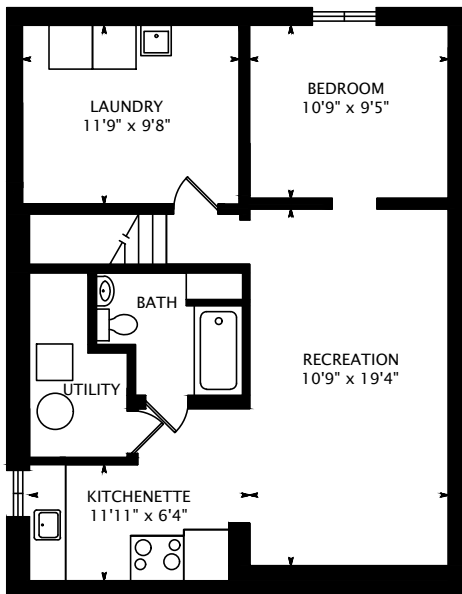
LOWER FLOOR 772 SQUARE FEET
