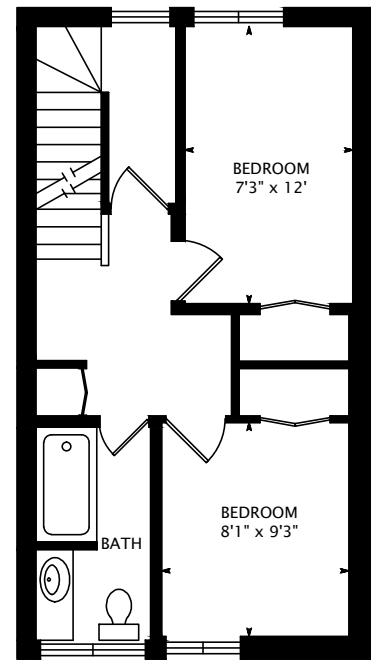
SECOND FLOOR 423 SQUARE FEET
