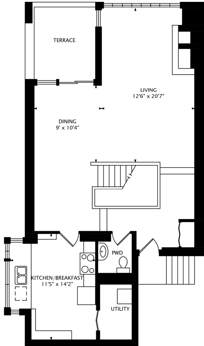
MAIN FLOOR 909 SQUARE FEET
